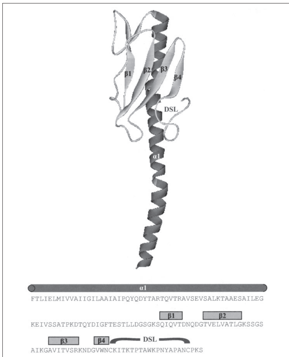
FIGURE 1. Primary and tertiary structure of 1244 pilin. Strain 1244 pilin tertiary structure was derived from homology modeling. Predicted \alpha -helix, \beta -sheets, and DSL are labeled on the model and above the corresponding amino acid sequence of mature 1244 pilin.
