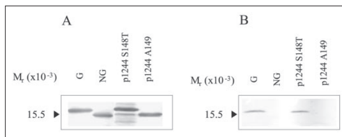
FIGURE 3. Western blot analysis of P. aeruginosa 1244 mutant pilins. Western blot of 1244 pilin produced by P. aeruginosa 1244N3/p1244 S148T and 1244N3/p1244 A149 of cell extracts using anti-1244 pilin monoclonal antibody 5.44 (A) or anti-1244 pilin glycan monoclonal antibody 11.14 (B) as a probe. G is glycosylated 1244 pilin, and NG is nonglycosylated 1244 pilin. Pilin terminating in Thr rather than Ser was glycosylated (1244N3/p1244 S148T), whereas pilin terminating in Ala, where Ser 148 was the penultimate residue, was nonglycosylated.
