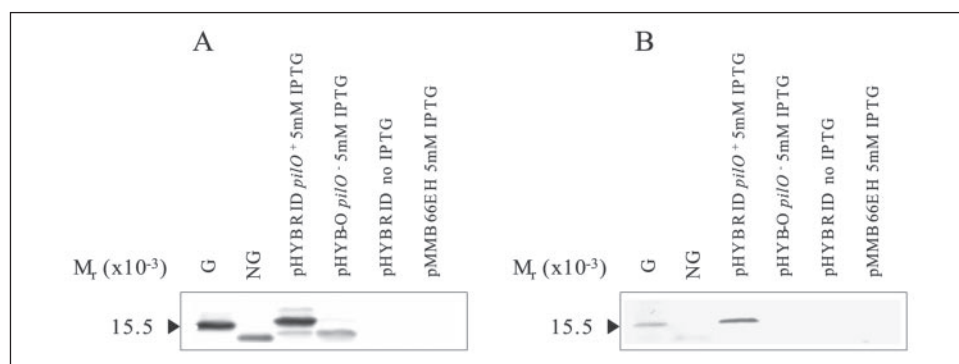
FIGURE 5. Western blot analysis of P. aeruginosa hybrid pilin. Western blot of pilin produced by P. aeruginosa 1244.47/pHYBRID and 1244.47/pHYB-O using anti-pilin polyclonal serum as a probe (A) or anti-1244 pilin glycan monoclonal antibody 11.14 (B) as a probe. G is glycosylated 1244 pilin, and NG is nonglycosylated 1244 pilin. Hybrid pilin was glycosylated in the presence of PilO (pHYBRID), whereas removal of PilO abrogated glycosylation (pHYB-O). The presence of a pilin band was found only in the presence of IPTG (A), and empty vector controls did not produce a band (pMMB66EH).
