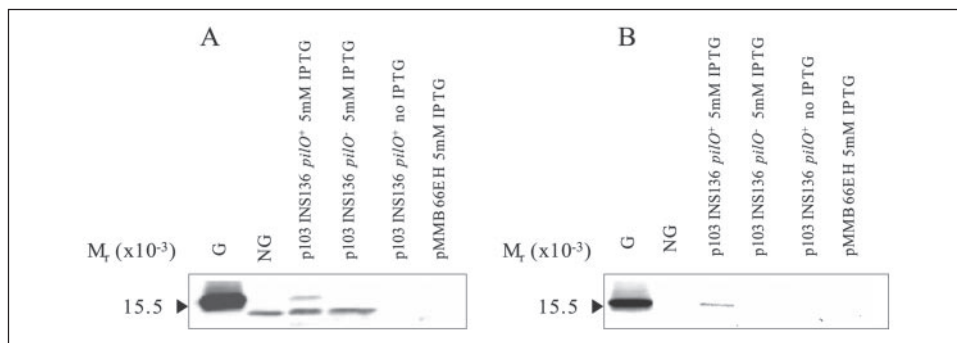
FIGURE 8. Western blot analysis of PA103 mutant pilin with insertion. Western blot of pilin produced by P. aeruginosa 1244.47/p103 INS136 in the presence of PilO (pUCP26 pilO ) or without PilO (pUCP26) using anti-pilin polyclonal serum as a probe (A) or anti-1244 pilin glycan polyclonal serum (B) as a probe. G is glycosylated 1244 pilin, and NG is nonglycosylated 1244 pilin. Pilin encoded by p103 INS136 was glycosylated in the presence of PilO, whereas removal of PilO abolished glycosylation. The presence of a pilin band was consistent with the presence of IPTG (A), and empty vector controls did not produce a band (pMMB66EH).
