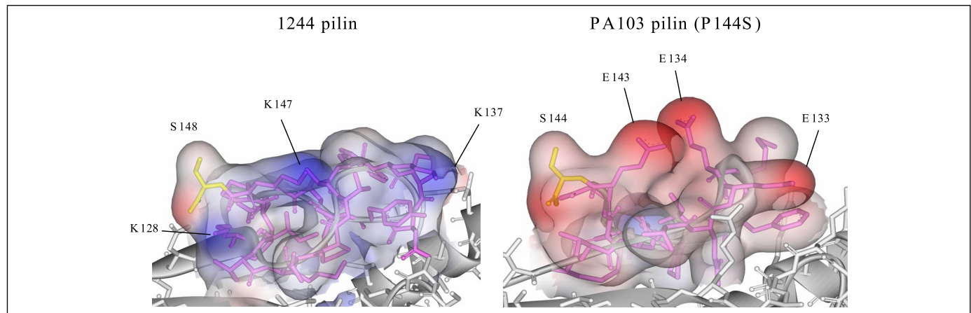
FIGURE 7. Predicted surface properties of the strain 1244 and PA103 pilin DSLs. Tertiary structures of 1244 pilin and PA103 (P144S) pilin generated by homology modeling. The residues of the DSL and tail are pink, and the C-terminal residue is yellow. Molecular surface of the DSL was generated and displayed in terms of Gasteiger charges where blue is positive and red is negative.
