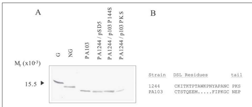
FIGURE 4. Western blot analysis of P. aeruginosa PA103 mutant pilins. Western blot of pilin produced by P. aeruginosa 1244/pSD5, 1244/p103 P144S, and 1244/p103 PKS using anti-PA103 pilin monoclonal antibody 2.97 as a probe (A). G and NG are glycosylated and nonglycosylated pilin standards, respectively, on a separate blot that was probed with anti-1244 pilin monoclonal antibody, 5.44. Wild type PA103 pilin (pSD5), PA103 pilin with residue Pro 144 (p103 P144S) mutated to Ser, as well as PA103 pilin with residues Asn 142 , Glu 143 , and Pro 144 mutated to that of 1244 pilin, Pro, Lys, and Ser, respectively (p103 PKS) were all nonglycosylated in the presence of PilO. The amino acid sequences of the DSL and tail regions of strains 1244 and PA103 pilin were aligned for comparison (B).
