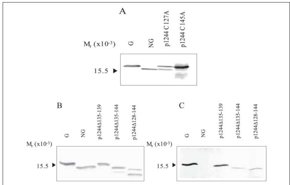
FIGURE 6. Western blot analysis of P. aeruginosa 1244 mutant pilins with Cys mutation or DSL deletion. Western blot of pilin produced by P. aeruginosa 1244N3/p1244 C127A and 1244N3/p1244 C145A using anti-1244 pilin monoclonal antibody 5.44 as a probe (A). Western blot analysis of pilin produced by P. aeruginosa 1244N3/p1244 \Delta 135–139, 1244N3/p1244 \Delta 135–144, and 1244/p1244 \Delta 128–144 using anti-1244 pilin monoclonal antibody 5.44 as a probe (B) or anti-1244 pilin glycan monoclonal antibody 11.14 (C) as a probe. G is glycosylated 1244 pilin, and NG is nonglycosylated 1244 pilin. All of the mutants produced some glycosylated pilin; however, p1244 C127A (A), p1244 \Delta 135–144, and p1244 \Delta 128–144 (B) produced some nonglycosylated pilin.
