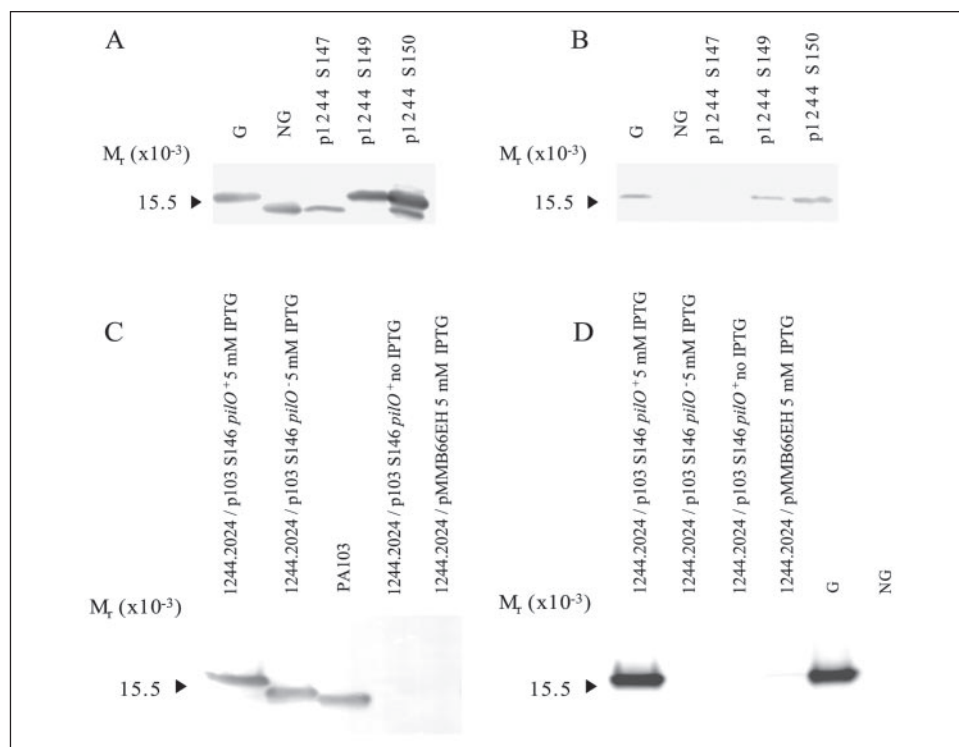
FIGURE 9. Western blot analysis of mutant pilins with altered tail lengths. Western blot of pilin produced by P. aeruginosa 1244N3/p1244 S147, 1244N3/p1244 S149, and 1244N3/p1244 S150 using anti-1244 pilin monoclonal antibody 5.44 as a probe (A) or anti-1244 pilin glycan monoclonal antibody 11.14 (B) as a probe. G is glycosylated 1244 pilin, and NG is nonglycosylated 1244 pilin. Pilin with longer tails were glycosylated (S149 and S150), whereas pilin with a shortened tail region was not glycosylated (S147). Western blot of pilin produced by P. aeruginosa 1244.2024/p103 S146 in the presence of PilO (pUCP26 pilO ) or without PilO (pUCP26) using anti-PA103 pilin monoclonal antibody 2.97 as a probe (C) or anti-1244 pilin glycan polyclonal serum (D) as a probe. Pilin encoded by p103 S146 was glycosylated in the presence of PilO, whereas removal of PilO eliminated glycosylation. The presence of a pilin band was consistent with the presence of IPTG (A), and empty vector controls did not produce a band (pMMB66EH). Pilin produced by 1244.2024/p103 S146/pUCP26 was nonglycosylated; however, it has a higher molecular weight than wild type PA103 pilin because the leader sequence was not cleaved, and this mutant pilin had two additional alanines in the tail region.
